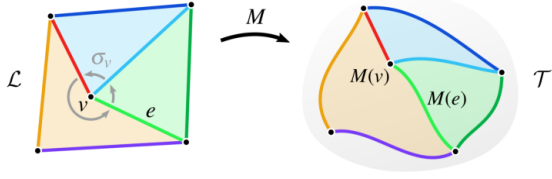
Figure 5: Vertices and edges of a layout \mathcal{L} are mapped to points and paths on a target surface \mathcal{T} via an embedding M . Embeddings are injective and preserve the cyclic ordering \sigma_v of edges around each layout vertex v .
