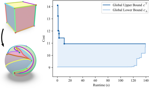
Figure 7: Progression of global upper bound c^+ and global lower bound c_- over the course of an optimization (here: embedding a cube layout into a sphere with random target vertex positions). The optimal solution is already found after 11 s. Optimality is proven after 139 s.
